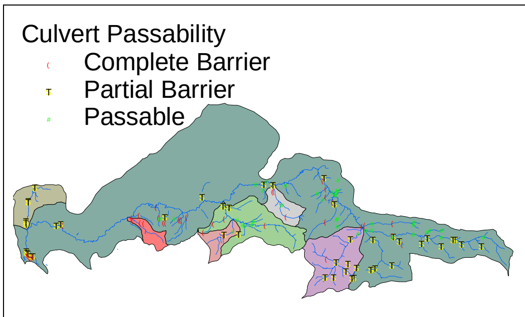
Figure 3-89: Culverts and Their Ratings for Passability in Johnson Creek
