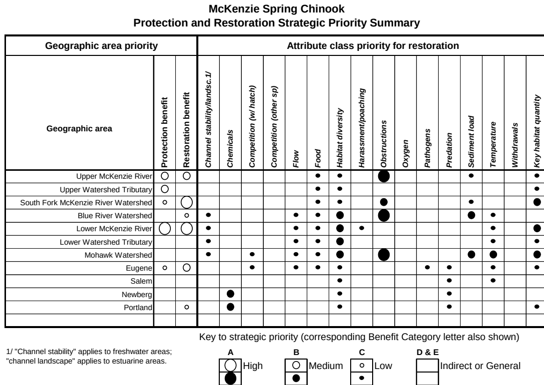
Figure 3-100: Aquatic and Riparian Protection and Restoration Priorities by EDT Attribute Class for McKenzie River Spring Chinook
