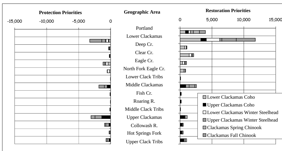
Figure 3-36: Protection and Restoration Priorities for Each Geographic Area in the Clackamas River in Regard to Abundance of All Six Focal Populations
