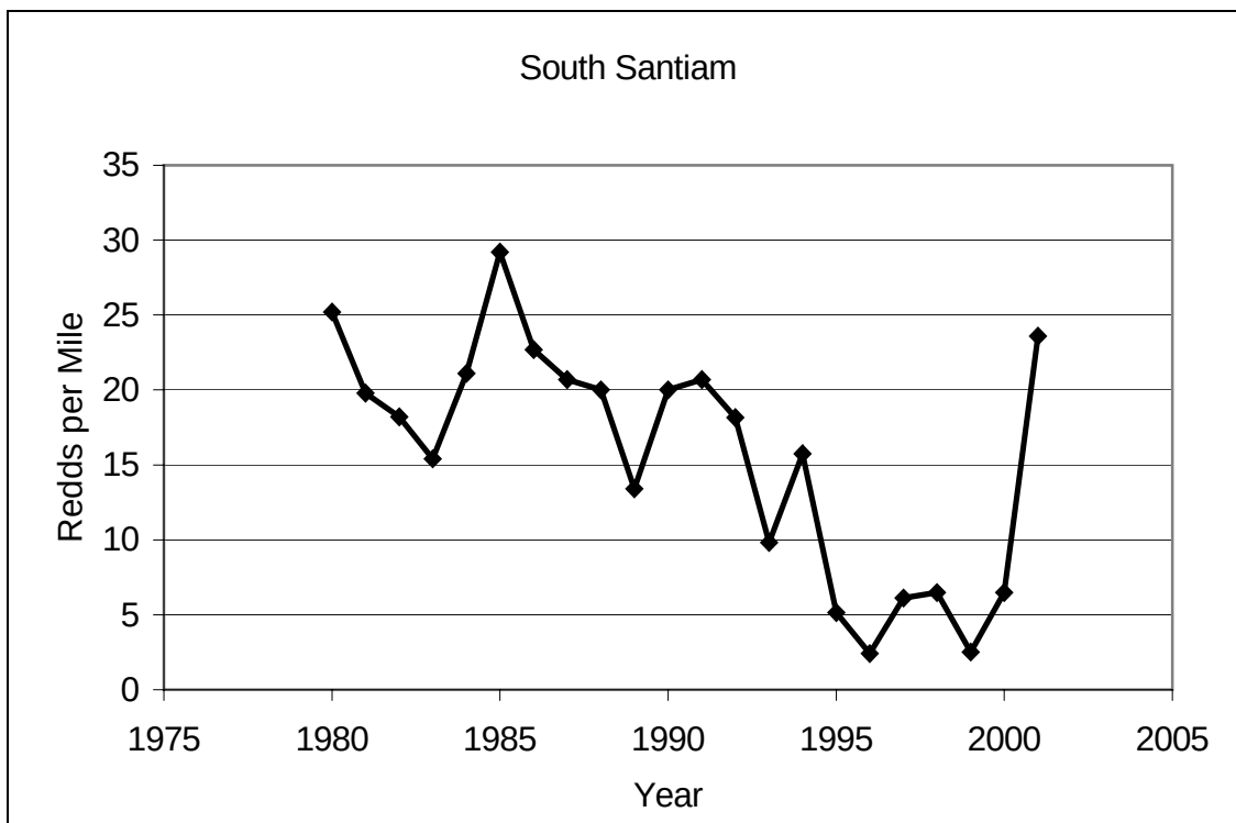
Figure 3-29: Redd Surveys of Winter Steelhead in the South Santiam Below Foster Dam
