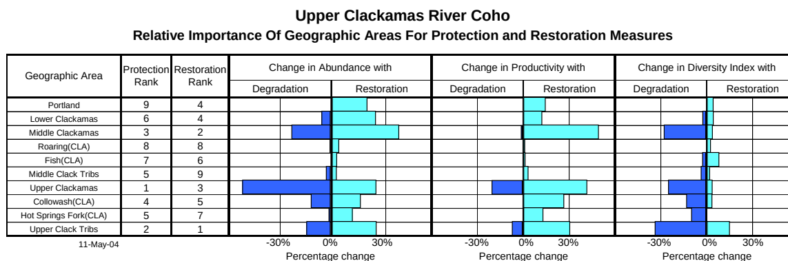
Figure 3-53: Upper Clackamas River Coho Habitat Priorities
