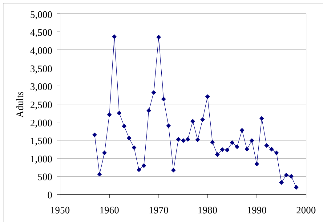
Figure 3-43: Abundance of Winter Steelhead at North Fork Dam
