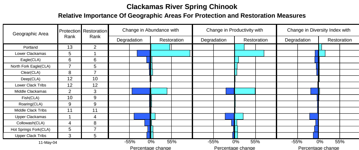
Figure 3-61: Clackamas River Spring Chinook Habitat Priorities
