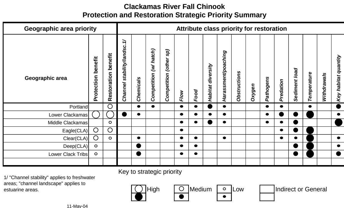
Figure 3-51: Clackamas River Fall Chinook Habitat Attribute Effects
