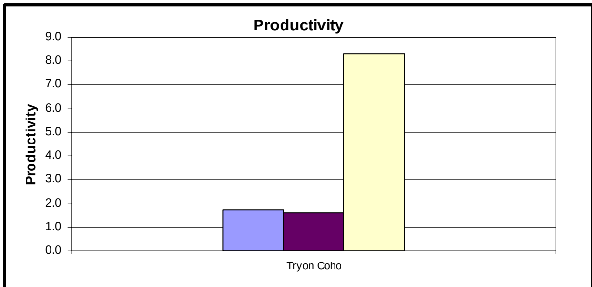
Figure 3-105: Estimated Fish Productivity Potential as a Function of Habitat in the Current and Reference Conditions for Tryon Creek Subbasin Coho Population
